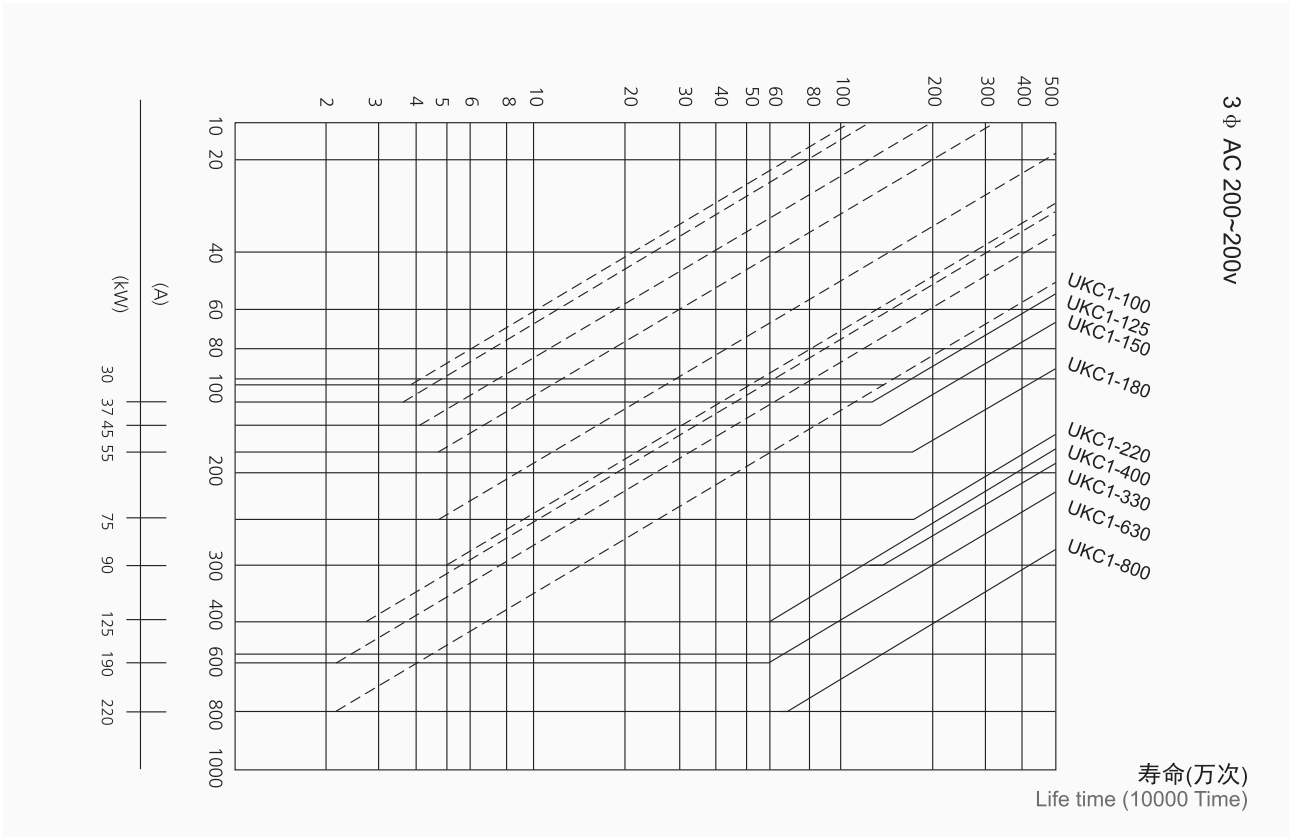
电气寿命曲线图(UKC1-100-800) The electrical life time(UKC1-100-800)
