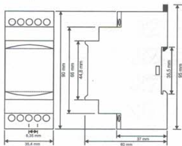
Dimensions for DT-321DIN / DT-322DIN
