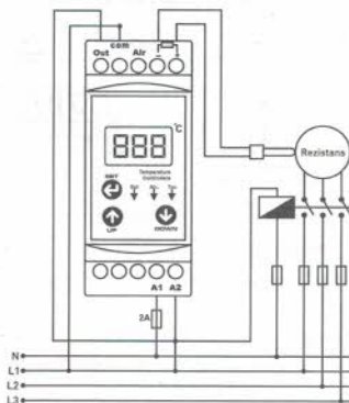
Connection Diagram for DT-321DIN / DT-322 DIN
