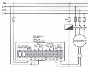
Connection Diagram for DT-321 / DT-322
